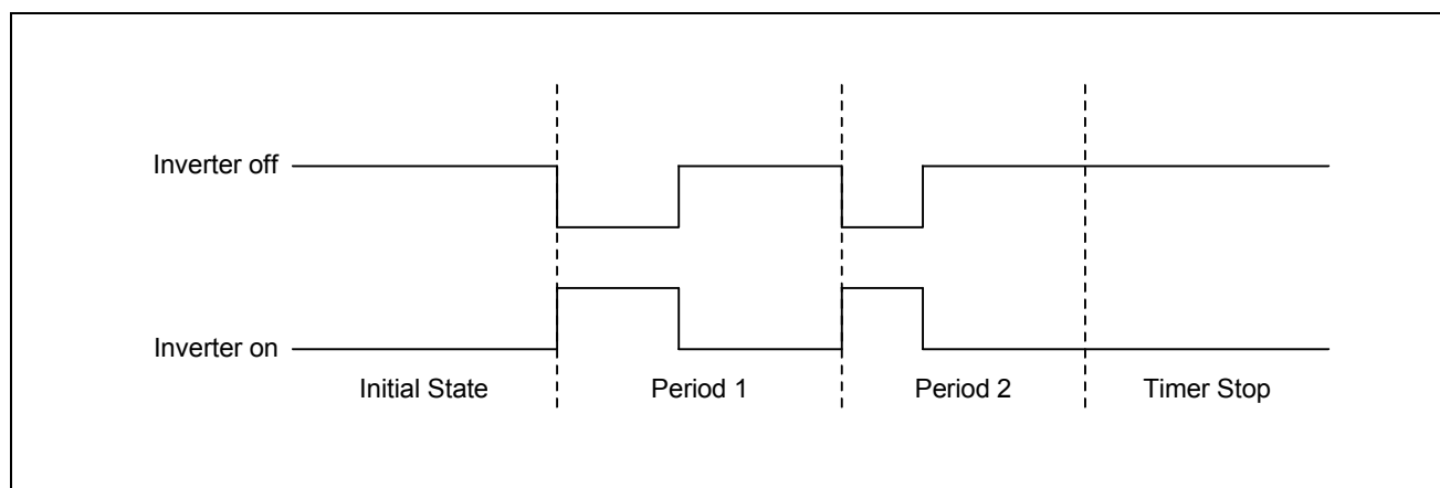
Figure 10-6. Inverter On/Off
